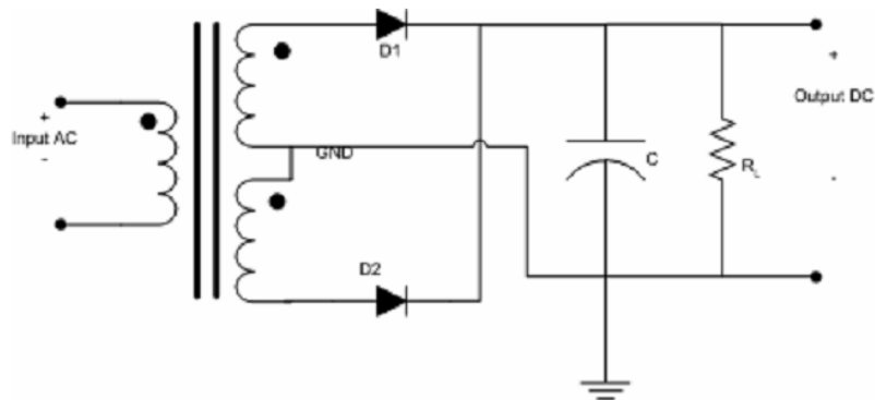
Figure 3.4: Full-wave Rectifier [3]
