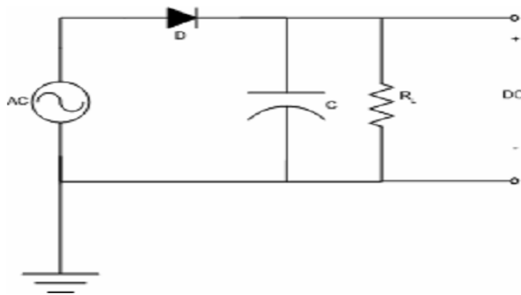
Figure 3.2: Peak Detector
