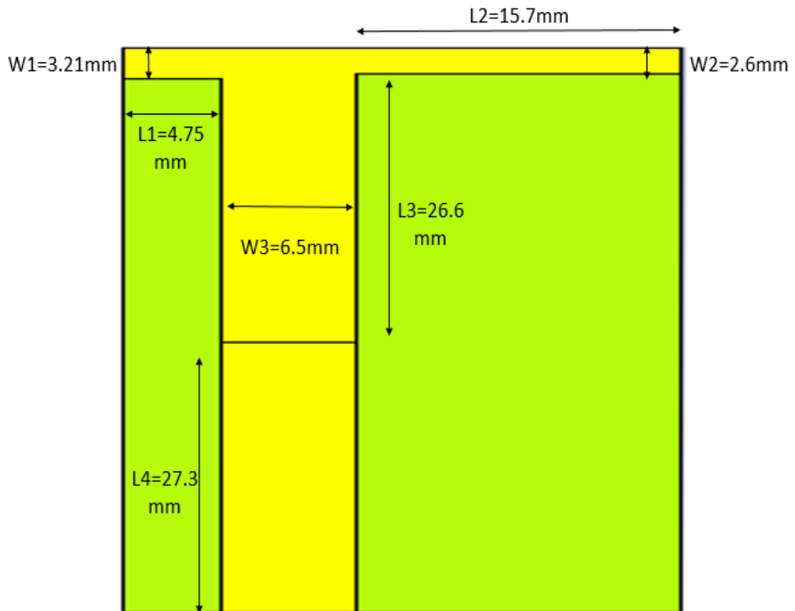
Figure 4.9: matching circuit layout for seven stage rectifier
